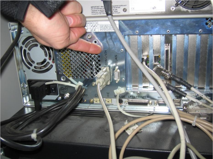
On the back side of the Siemens PC the data cable from the scanner is attached (COM 2)
